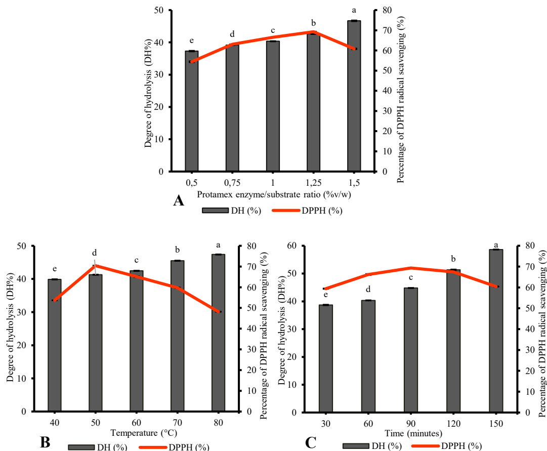
Fig. 1. The effects of hydrolysis conditions of APC by protamex enzyme.
