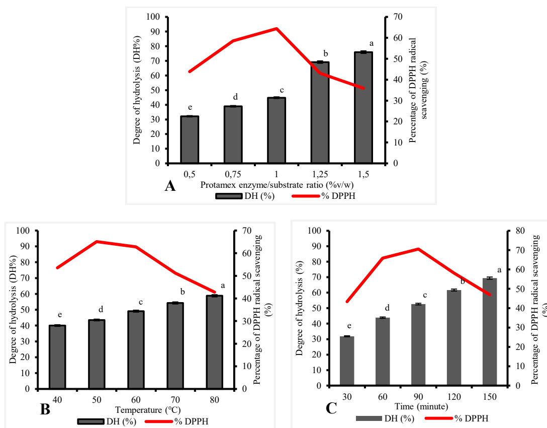
Fig. 3. The effects of hydrolysis conditions of R-PE by protamex enzyme.
