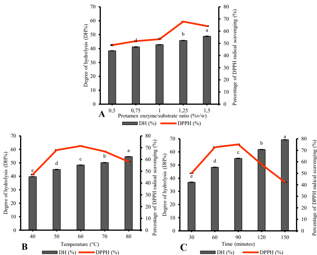
Fig. 2. The effects of hydrolysis conditions of C-PC by protamex enzyme
